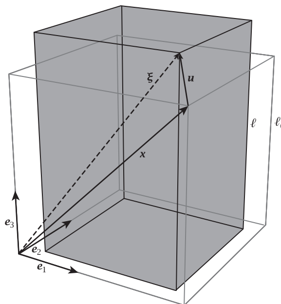
Figure 2 A deformed configuration of a solid body that was a cube in its reference configuration.
