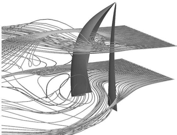
Figure 5 Streamlines around mainsail and gennaker.
