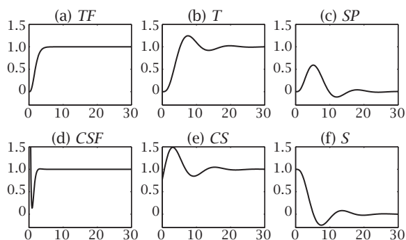
Figure 3 Step responses for P(s) = (s+1)^{-4} and C(s) = 0.8(0.5s^{-2}+1) when TF = (0.5s+1)^{-4} .
