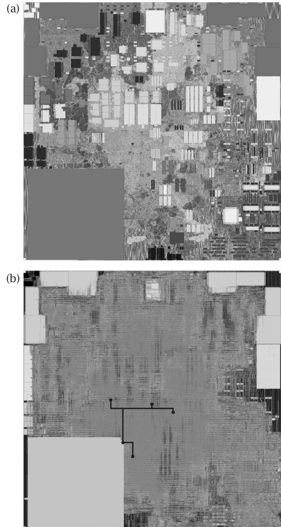
Figure 1 (a) Placement and (b) routing of a chip with 4 496 492 circuits and 5 091 819 nets, with 762 meters of wires. Large rectangles are pre-designed units, e.g., memory arrays or microprocessors. A Steiner tree connecting the five pins of one net is highlighted in (b).
