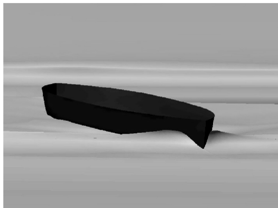
Figure 7 Free-surface flow around a rowing boat.
