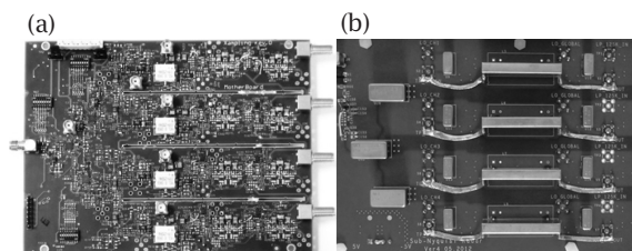
Figure 1 Sub-Nyquist hardware prototypes for (a) cognitive radio and (b) radar.
