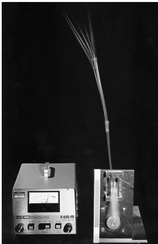
Figure 2 An inverted triple pendulum.
