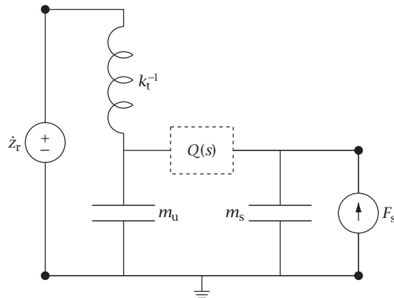
Figure 5 The equivalent electrical circuit for the quarter-car model.
