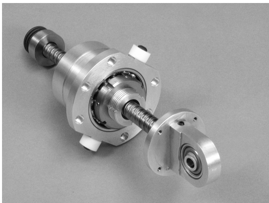
Figure 6 A ballscrew inerter made in the University of Cambridge engineering department in 2003, with flywheel removed.
