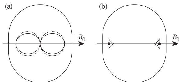
Figure 2 (a) Phase velocities and (b) group velocities for the various MHD waves with an imposed magnetic field as shown. Solid lines denote the fast and slow waves; the Alfvén waves are denoted by the dashed lines in (a) and the solid circles in (b). The ratio of Alfvén to sound speeds (or the inverse ratio; the picture is unaltered) is 0.8.
