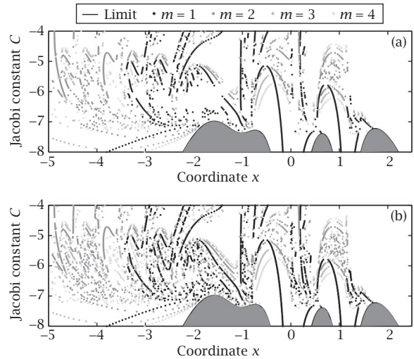
Figure 3 Symmetric periodic orbits ( m denotes the multiplicity of the periodic orbit) in the most chaotic zone of the (7 + 2) -ring problem using (a) double and (b) quadruple precision. Note the “gaps” in the double precision plot. (Reproduced by permission of Roberto Barrio.)
