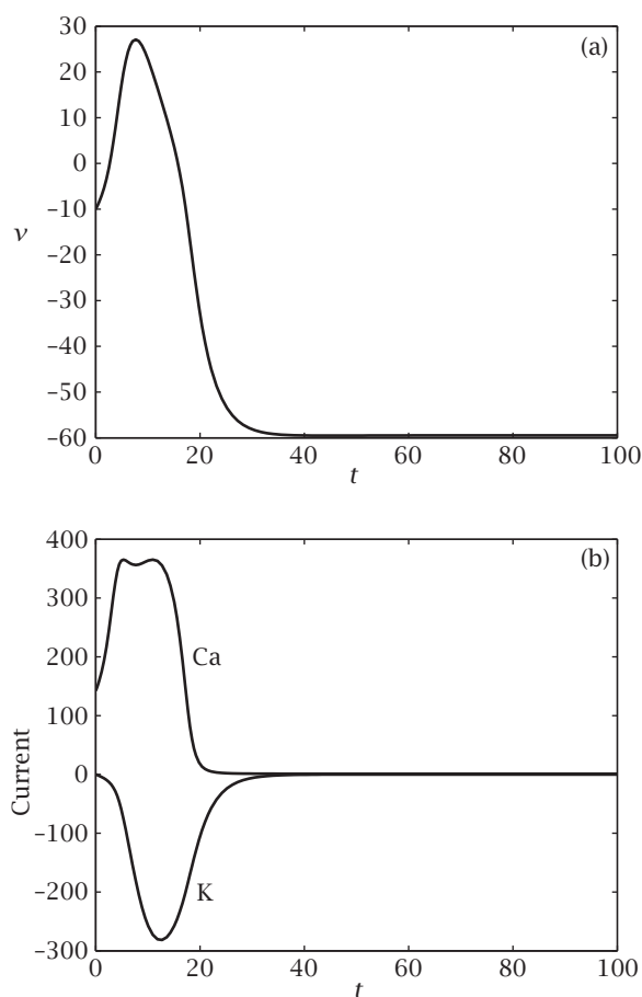
Figure 3 Solution to the Morris-Lecar model with v initialized to -10 mV: (a) voltage; (b) K^+ and Ca^{2+} currents. The solution exhibits an initial bump (or crest) before decaying to rest.
