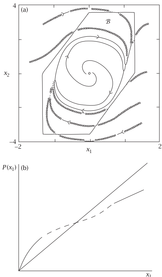
Figure 5 (a) An annular trapping region B and the limit cycle of the van der Pol equation (13) with \mu = 1 . (b) The Poincaré map for equation (13) expands lengths for x_1 small and contracts them for x_1 large, implying the existence of at least one fixed point corresponding to a periodic orbit.
