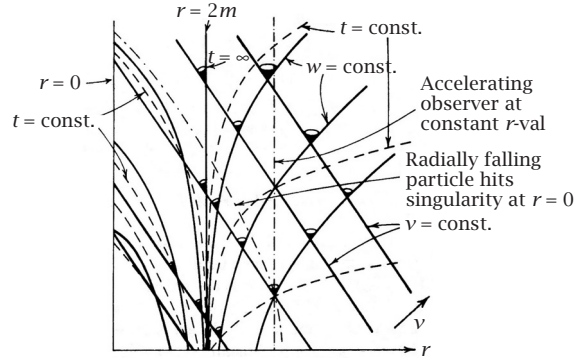
Figure 1 Radial null geodesics and local light cones in the Schwarzschild solution in Eddington-Finkelstein coordinates (reproduced from Hawking and Ellis (1973), with permission).
