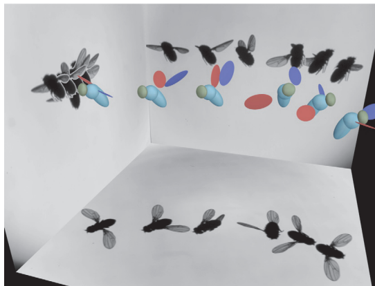
Plate 11 (VL5). A fruit fly making a sharp yaw turn of 120^\circ in about 20 wing beats, or 80 ms. The wing hinge acts as if it is a torsional spring. To adjust its wing motion, the wing hinge shifts the equilibrium position of the effective torsional spring, and this leads to a slight shift of the angle of attack of that wing. The asymmetry in the left and right wings creates a drag imbalance that causes the insect to turn. To turn 120^\circ , the asymmetry in the wing angle of attack is only about 5^\circ or so. From A. J. Bergou, L. Ristroph, J. Guckenheimer, I. Cohen, and Z. J. Wang (2010), Fruit flies modulate passive wing pitching to generate in-flight turns, Physical Review Letters 104:148101.
