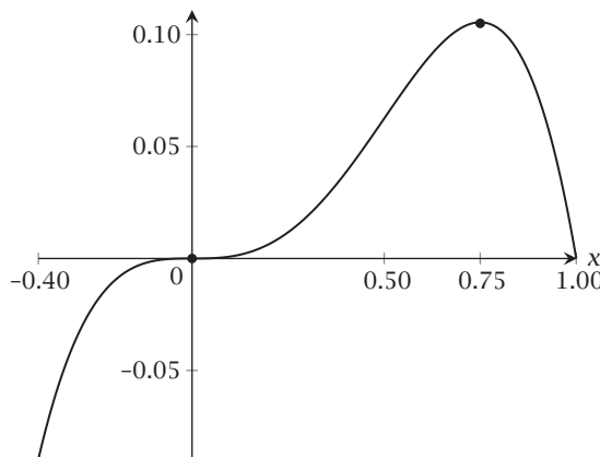
Figure 6 The function f(x) = x^3 - x^4 with a saddle point at x = 0 and a maximum at x = 3/4 .
