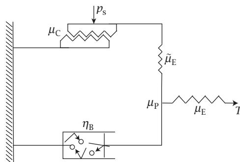
Figure 5 Slide block/spring/dashpot analogue of visco-elastoplasticity.
