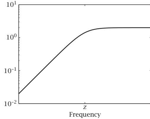
Figure 9 Limitation from unstable zero. The sensitivity function S(i\omega) = (1 + P(i\omega)C(i\omega))^{-1} should be small for low frequencies in order to reject disturbances and follow reference signals at least on a slow timescale. However, if P(z) = 0 , z > 0 , then no stabilizing controller C can push the sensitivity function |S(i\omega)| entirely below the curve above. As a consequence, the unstable zero z puts an upper limit on the speed of disturbance rejection in the closed-loop system.
