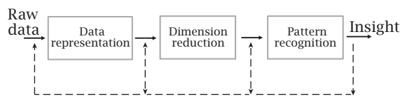
Figure 1 A schematic showing the overall process of data analysis.
