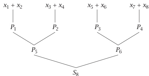
Figure 1 A binary tree for pairwise summation, with partial sums P_i .
