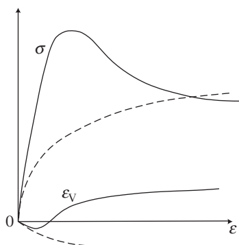
Figure 4 Schematic of triaxial stress/dilatation-strain curves for initially dense (solid curves) and loose (dashed curves) sands.
