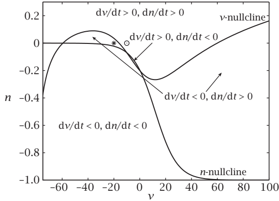
Figure 4 The v - and n -nullclines divide the v - n space into regions where v and n are increasing or decreasing.
