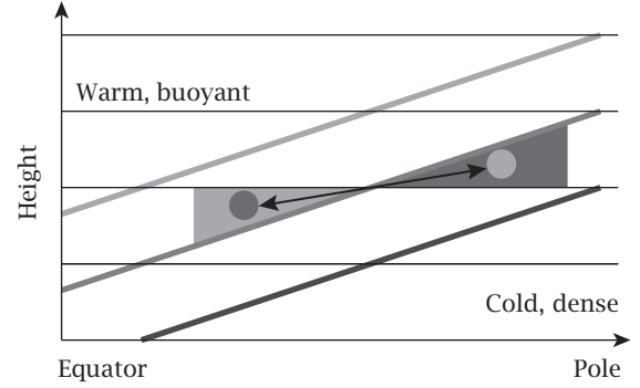
Figure 5 Schematic indicating parcel trajectories relative to sloping surfaces of constant potential temperature (gray lines) within a wedge of instability (filled region) for a baroclinically unstable disturbance in a rotating frame.
