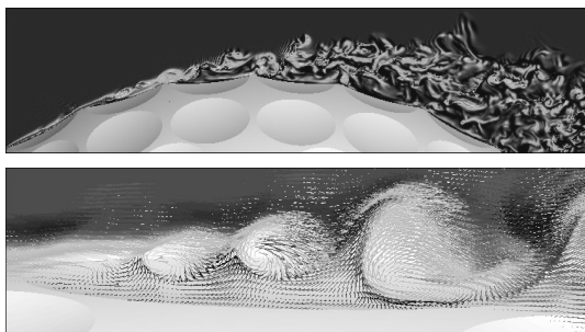
Figure 5 Simulation of flow over dimples.
