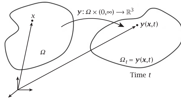
Figure 1 The Lagrangian description of motion.
