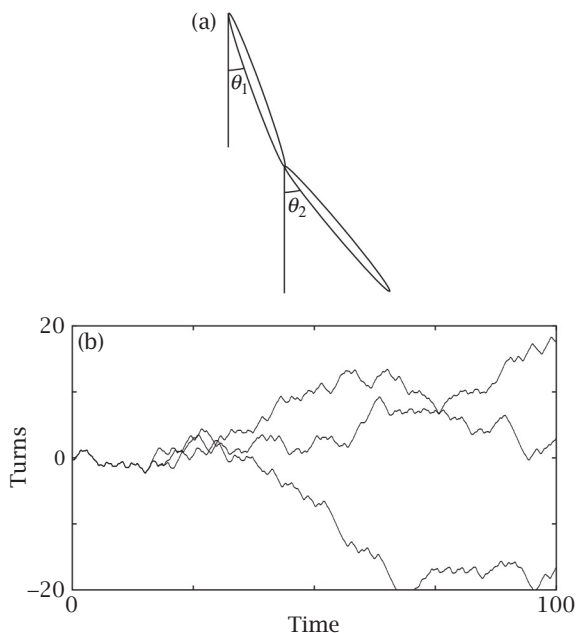
Figure 1 (a) The double pendulum. (b) The numbers of full turns, \theta_2 , executed by three different orbits released from rest with \theta_1(0) = 90^\circ , \theta_2(0) = -90^\circ , and \theta_2(0) = -(90 \pm 10^{-6})^\circ .
