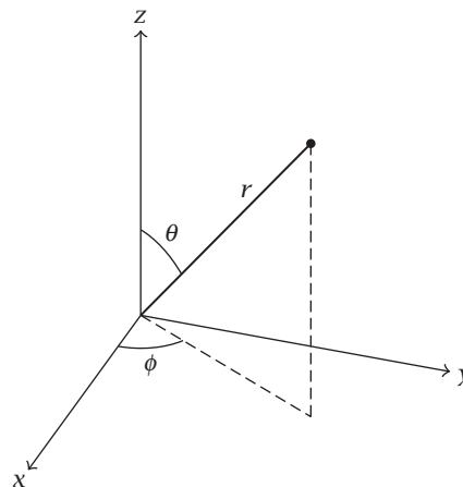
Figure 2 Spherical coordinates.
