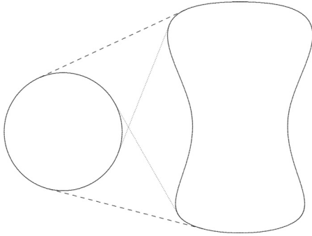
Figure 5 Calculated common tangents to a pair of curves.
