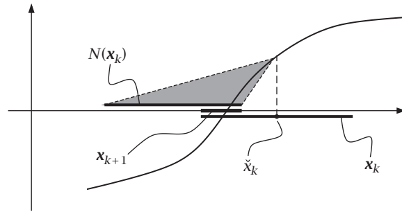
Figure 2 One iteration of the interval Newton method.
